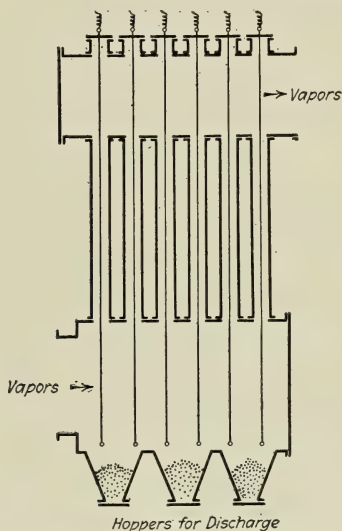
FIG. 72.—Cottrell Electrical Precipitator.
